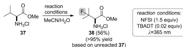
Scheme 2. Site-selective fluorination of sclareolide, benzaldehyde, and amino acid derivatives. The yields for 35 , 36 , and 38 are calculated from 1 H NMR spectra recorded on crude reaction mixtures with the addition of an internal standard.
